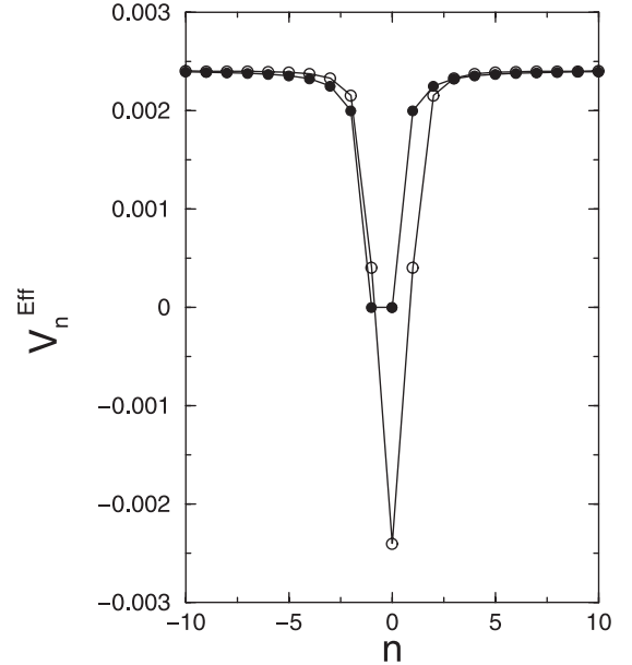
Fig. 7. Effective potential V_n^{Eff} , versus site number, n , for the interfaced piecewise system (dots) and for the single inverted dipole system (open circles).
