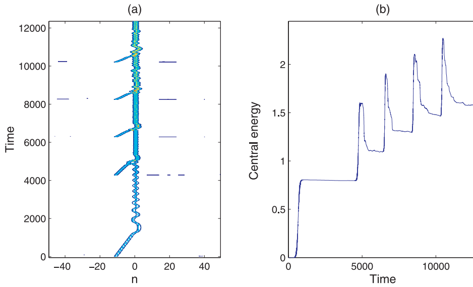
Fig. 10. (a) Contour plots for the evolution of five breathers launched towards the interface with different translational kinetic energies. The breathers are trapped at the interface increasing the accumulated energy density ( \lambda = 0.05; 0.07; 0.15; 0.19; 0.2 ). (b) Time evolution of the central energy.
