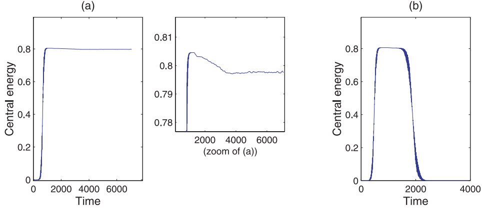
Fig. 5. Time evolution of the central energy corresponding to the collision processes: (a) in Figure 4a; (b) in Figure 4b. The central figure is a zoom of the left one.
