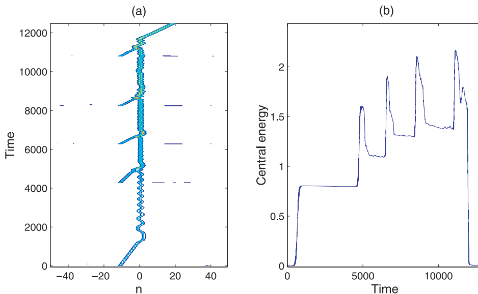
Fig. 11. (a) Contour plots for the evolution of five breathers launched towards the interface, with different translational kinetic energies ( \lambda = 0.05; 0.07; 0.15; 0.18; 0.14 ). After the last collision the accumulated energy is transmitted to the right side of the chain. (b) Time evolution of the central energy.
