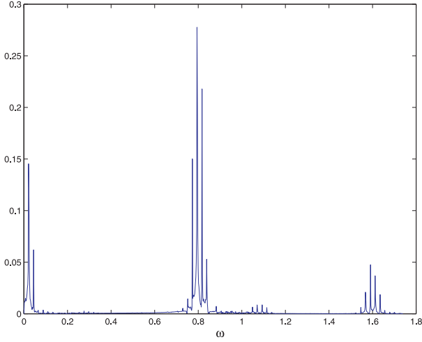
Fig. 6. Absolute values of the Fourier components of the trapped breather shown in Figure 4a calculated soon after the collision.
